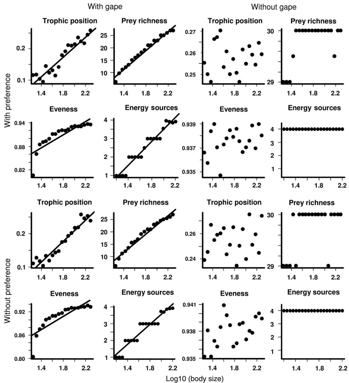
Figure 3. IBM evaluation of gape limitation and size preference as determinants of changes in trophic structure with body size. Gape limitation is identified as a necessary condition to reproduce the observed patterns, while size preference neither reproduces the patterns nor interacts with the effect produced by gape limitation.
