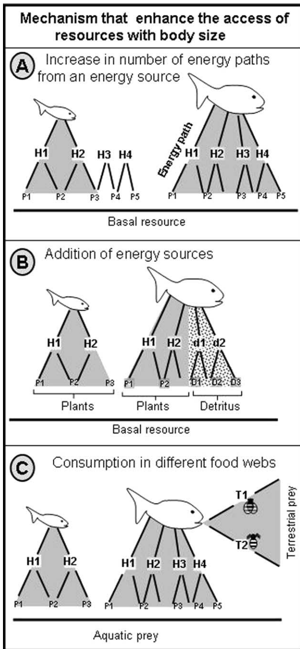
Figure 2. Conceptual explanation of the mechanisms that could allow a large predator to satisfy its energetic demand at higher trophic positions. (A) species richness is associated with standing biomass and resource flow, as a consequence, great prey richness implies a potential access to more resources. (B) the number of energy sources increases with body size, each source implies the incorporation of new resources increasing the total amount. (C) the incorporation of prey from other communities further increases the amount of resources.
