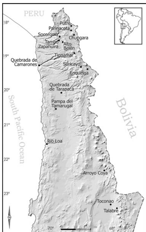
Figure 1 Map of northern Chile (Tarapacá and Antofagasta Regions) showing the localities sampled for small mammals in the altitudinal gradient from the coast to the Puna.
