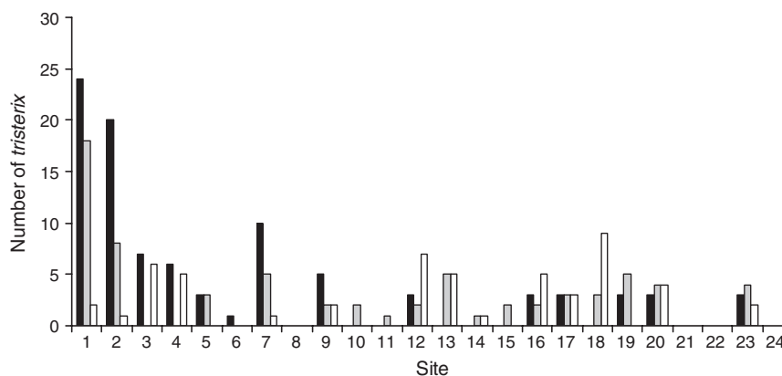
Fig. 2. Number of Tristerix corymbosus individuals by volume that represents age for each sample site. Sites 1–8 are from Llolelhue River, 9–16 are from Contra River, 17–20 are from fragments, and 21–24 are from continuous forests. Black bars represent older individuals, grey bars medium-age individuals and white bars young individuals.
