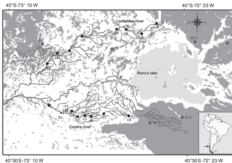
Fig. 1. Sample points of Dromiciops in Llollehue (LI) and Contra (C) rivers, with forest fragments (F, in grey) and continuous forest (CF, in white). The agricultural matrix is shown in white.
